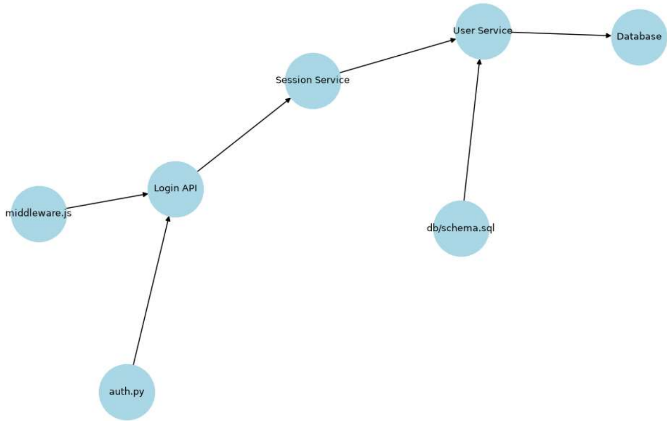
Repository Dependency Analysis
